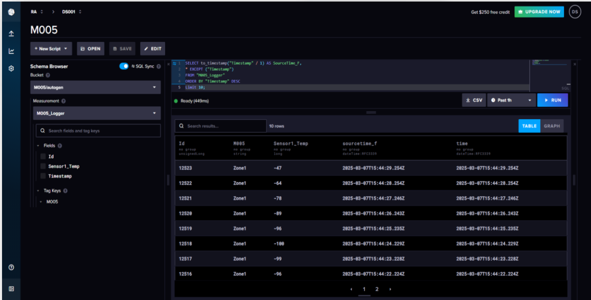
InfluxDB Cloud Serverless Storage Engine Version 3
